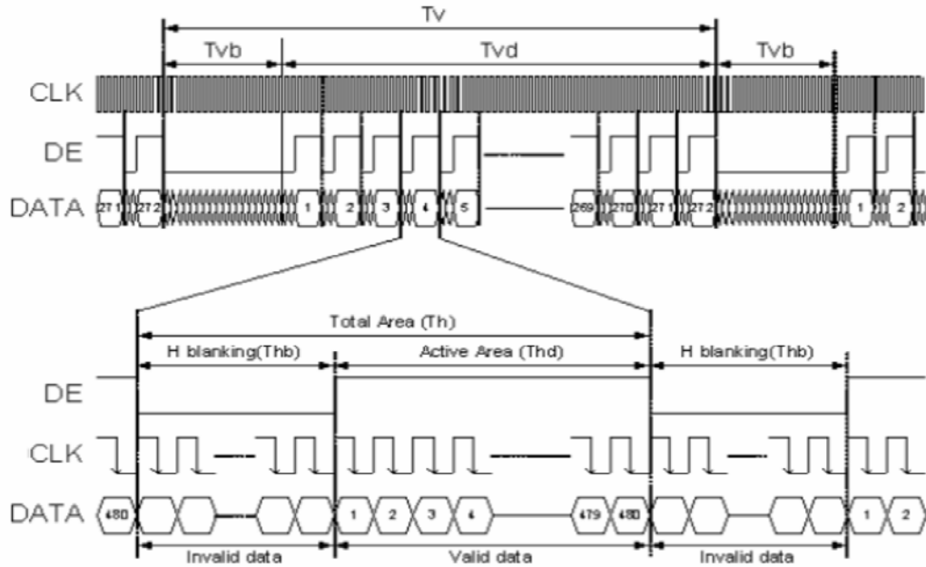
Parallel DE mode RGB input timing table
